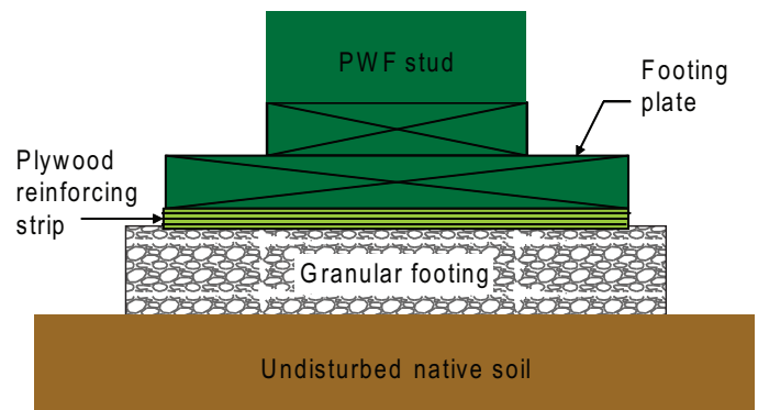
Figure C5.5.2.2-1 Plywood Reinforcing Strip
