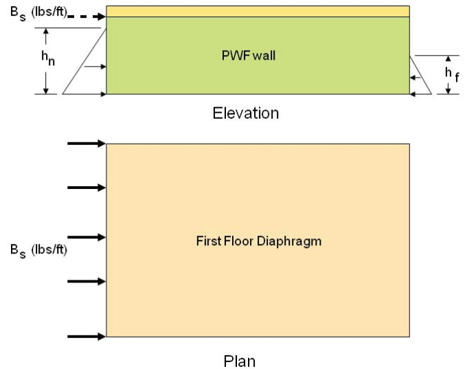
Figure C5.4.5.1 Net Resultant of Forces Due to Differential Backfill Height
