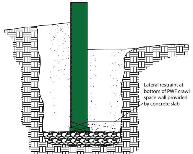
Figure C5.4.4.2 Concrete Slab to Resist Lateral Forces at the Bottom of a Crawl Space Wall
