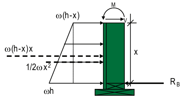
Figure C5.4-3 Calculating Shear at a Section “ x ” in the PWF Stud
