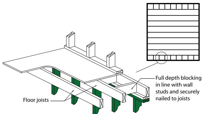
Figure C5.6.2.2 Blocking for PWF End Walls
